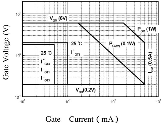
Fig 1. Gate Characteristics
