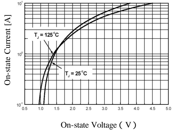
Fig 2. On-State Voltage
